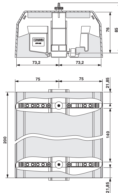
Dimensional drawing
